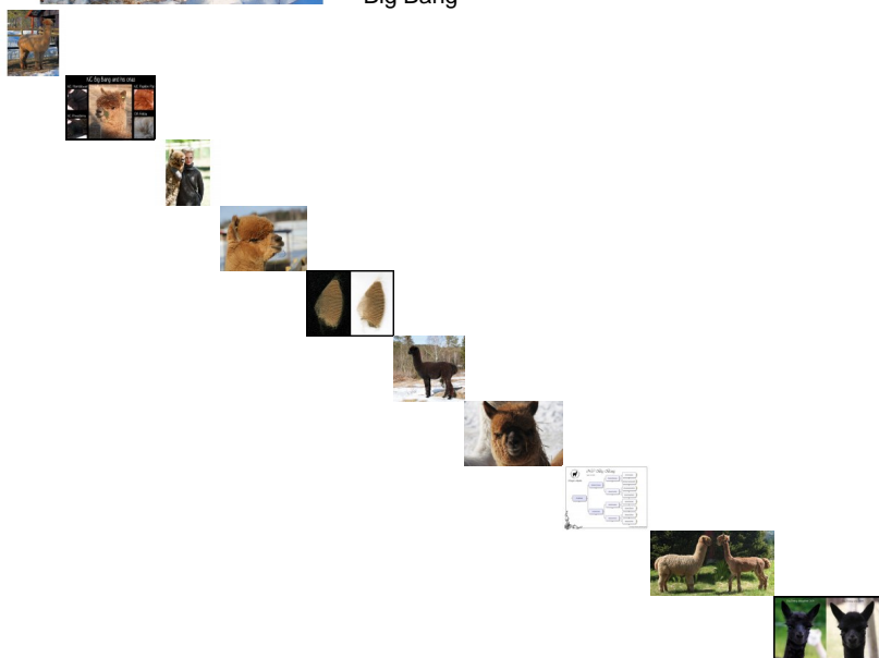
Big Bang
